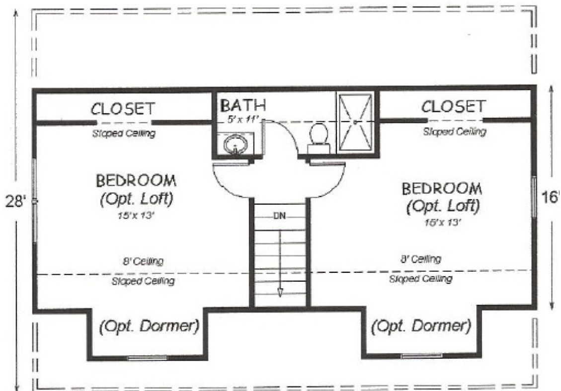
Second Floor
